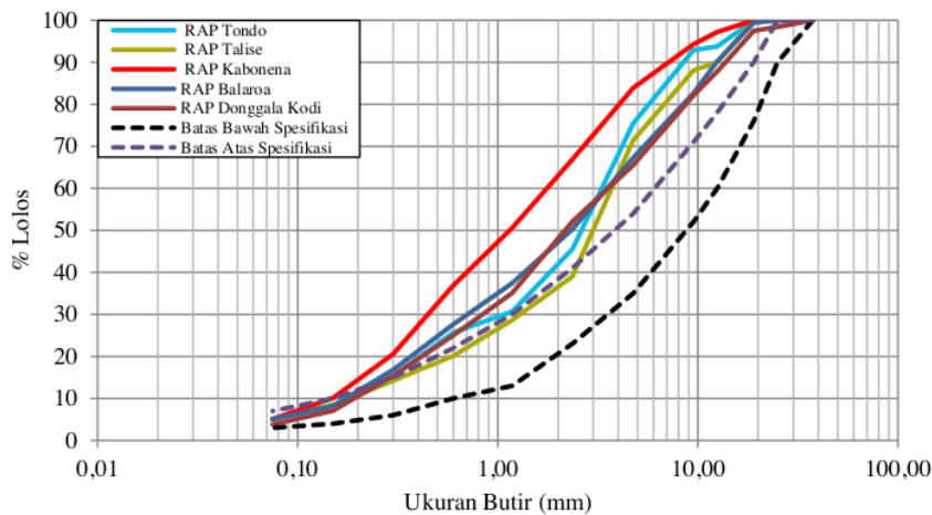
Gambar 3. Gradasi RAP terhadap campuran AC-Base
